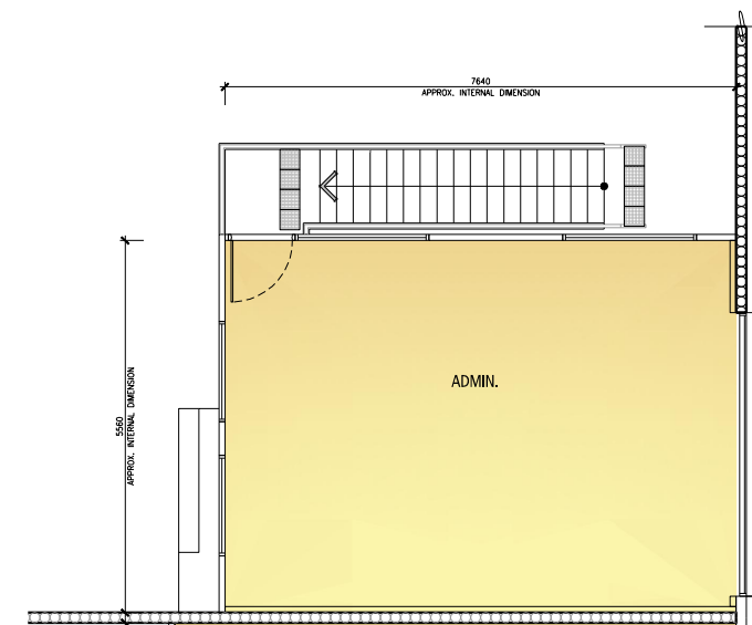
OFFICE 8 MEZZANINE PLAN SCALE: 1:50 @ B1
